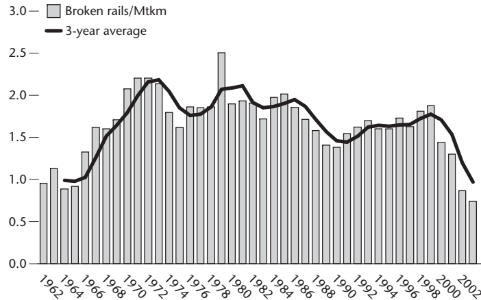
Figure 4 Number of broken rails Per million train kilometres (Mtkm)
